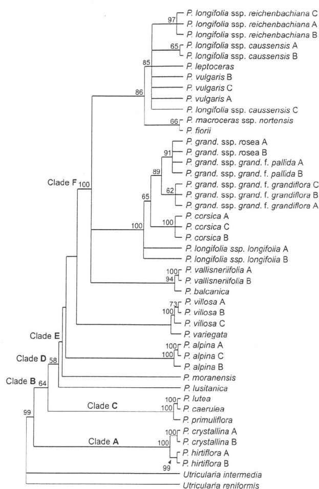
The major clades of Pinguicula are indicated. The letters after taxon names correspond to different sources of material as outlined in Table 1.
