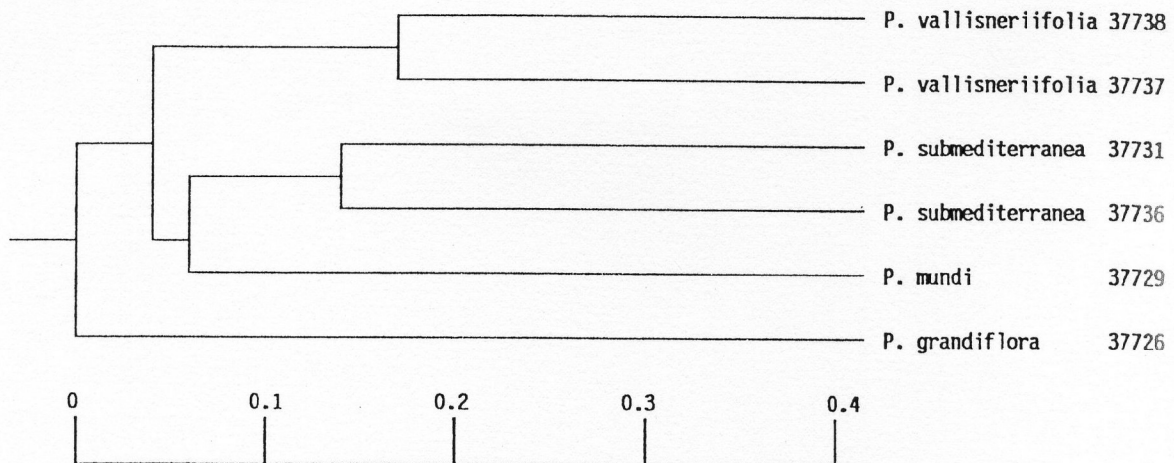
Fig. 5. Dendrogram generated by cluster (UPGMA) analysis of genetic distance values given in Table 6 showing relationships between different Pinguicula species
